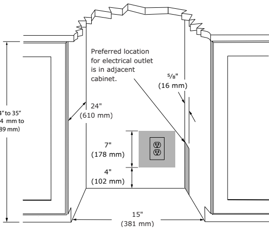
CABINET CUT-OUT
