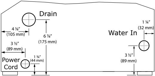
CABINET CUT-OUT
