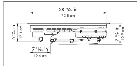
Fig. 5.2 Appliance dimensions front view
