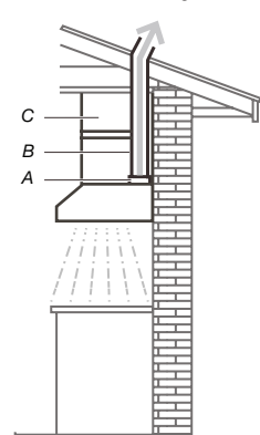
Vertical Discharge
