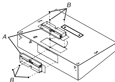
A. 3 1/4" x 10" (8.3 x 25.4 cm) rectangular vent damper B. 3.5 x 9.5 mm screws
