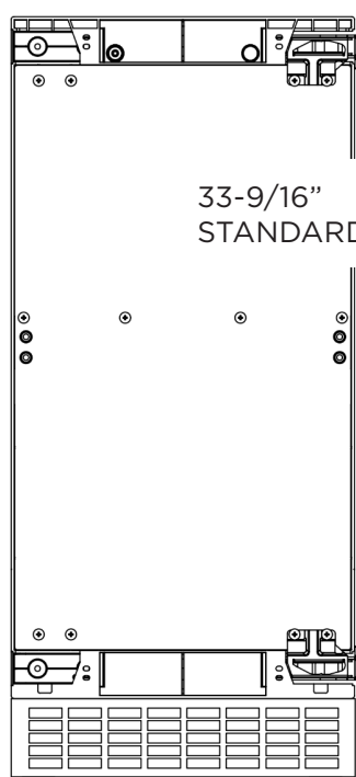
FRONT VIEW (WITHOUT PANEL)
